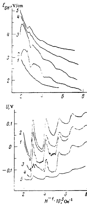
FIG. 8. Oscillations of U and E_{GH} recorded in a single experiment: T = 1.27^\circ \text{K} , \rho = 15 \Omega\text{-cm} . Intensities I [\text{cm}^{-2} \text{sec}^{-1}] : 1- 10^{17} , 2- 2 \cdot 10^{16} , 3- 2 \cdot 10^{15} , 4- 7 \cdot 10^{14} , 5- 2 \cdot 10^{14} .
