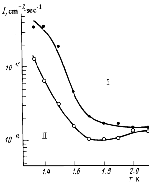
FIG. 6. Position of the maximum on the E_{GH}(I) and temperature dependence at H = 35 kOe (lower curve) and H = 28.5 kOe (upper curve), \rho = 30 \Omega\text{-cm} .
