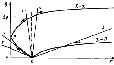
FIG. 9. Graphic solution of Eqs. (11) and (13). The lines 1 and 4 correspond to the inequality \epsilon > 2m^*s^2 , line 2 to the inequalities 2m^*s^2 > \epsilon > m^*s^2/2 , and lines 3 and 5 to the condition \epsilon < m^*s^2/2 .
