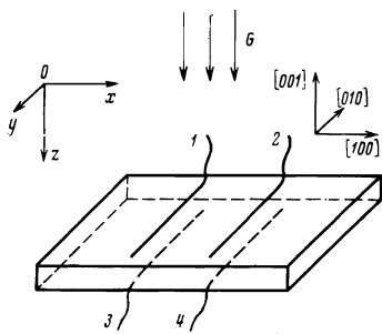
FIG. 1. Placement of contacts on the sample; G —light flux incident on the sample.
