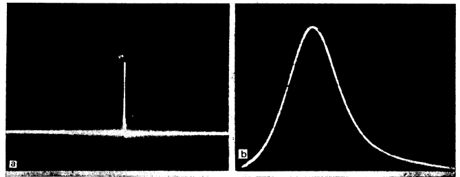
FIG. 3. Oscillograms of giant pulse. Sweep rates 20 μsec (a) and 50 nsec (b) per division.
