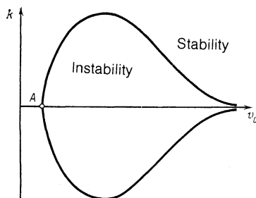
FIG. 3. Neutral-stability curve of a solitary surface wave over an uneven bottom. The point A corresponds to the value v_0 = 0.2 \sigma^{-4/3} R^{-2/3} .
