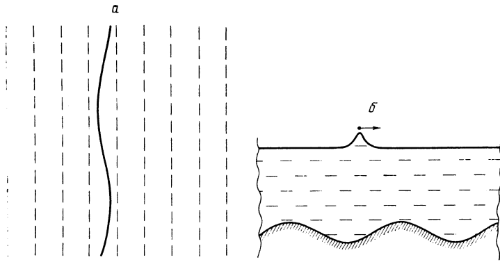
FIG. 1. Formulation of problem: propagation of a solitary wave over the surface of an ideal liquid in a basin with an uneven bottom: a) top view (solid line—soliton ridge, dashed—equal-depth line); b) side view.
