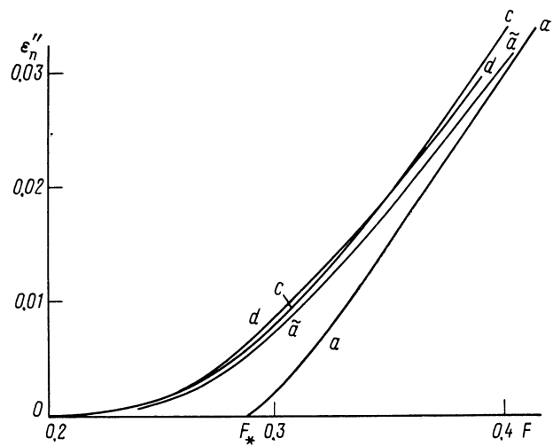
FIG. 1. Reduced width \varepsilon''_n = n^2 \Gamma_n for the |9,0,0\rangle with n = 10 . Curve a: 1/n approximation without allowance for barrier penetration, i.e., \varphi(a) \rightarrow 0 ; curve \bar{a} : 1/n approximation with allowance for barrier penetration [see (4.2)]; curve c: result of the PHA method (Ref. 21); curve d: 1/n approximation improved as in (4.7).
