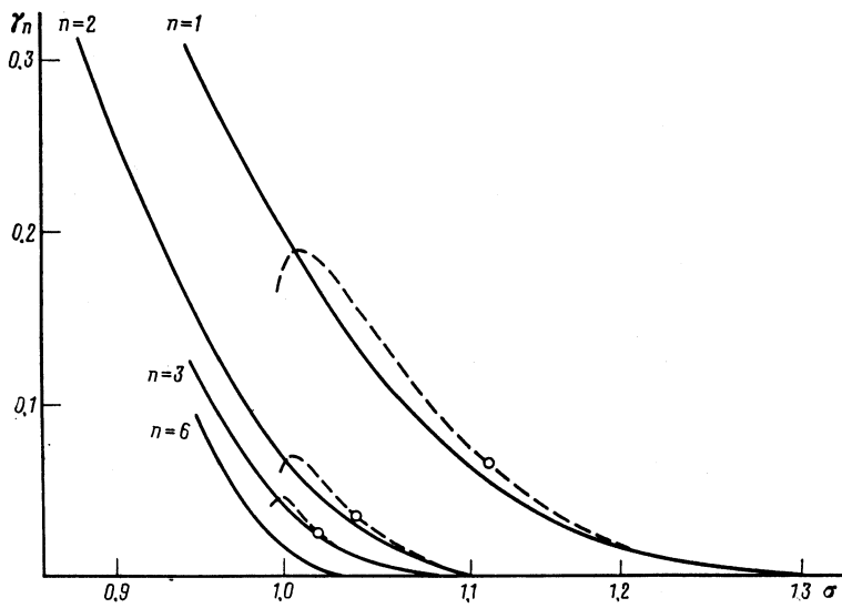
FIG. 2. Reduced width \gamma_n [see (3.10)] for ns levels in the potential (3.4). The points for which \alpha = 1 are denoted by \circ . The solid curves are from an exact calculation using (3.9), and the dashed curves are obtained from the Gamov formula (3.8); \sigma = (g/g_n)^{1/4} .
