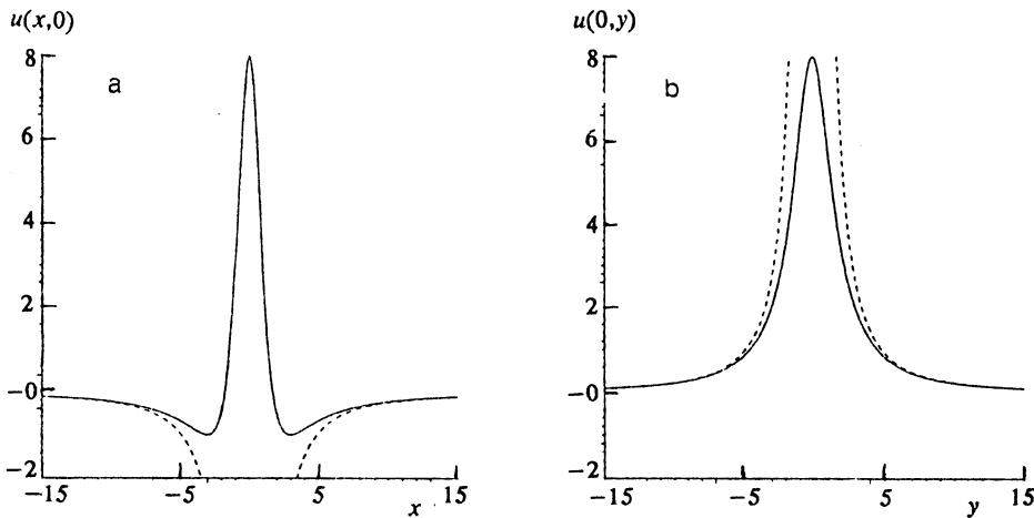
FIG. 1. The longitudinal (a) and transverse (b) cross-sections of a two-dimensional soliton (solid lines) and their linear asymptotic forms (dashed lines).
