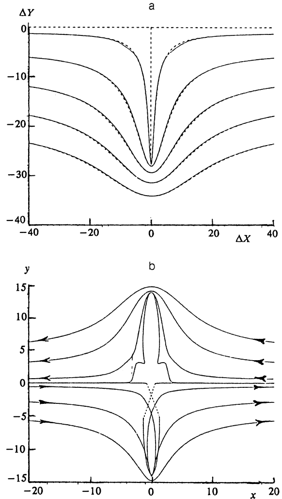
FIG. 3. a) The same as Fig. 2, but for \Delta V_x = 0, 5 ; \Delta V_y = 0 . b) The trajectories of two solitons in the exact solution.
