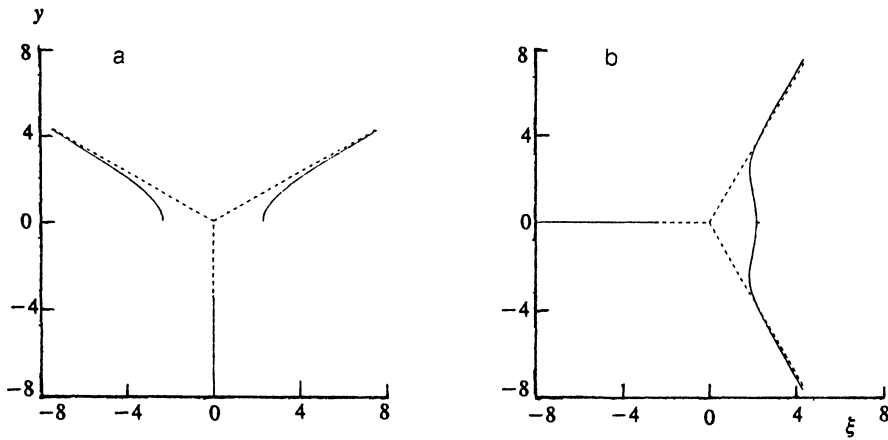
FIG. 6. The locations of three solitons which form a bound state in the approximate (4.1) (dashed traces) and the exact (4.2) (solid traces) solutions for two configurations relative to the mean velocity of motion.
