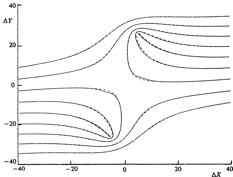
FIG. 2. The trajectories of the relative distances between soliton maxima in the exact solution (solid lines) and in the asymptotic approach (dashed lines) for asymptotic velocities: \Delta V_x=0, 5 ; \Delta V_y=0, 1 .
