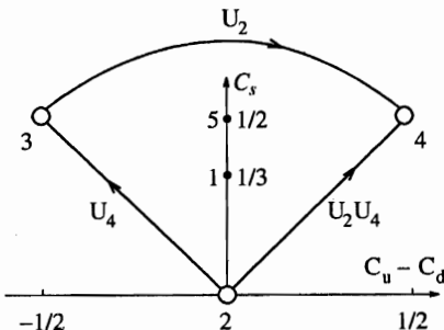
Fig. 1. Map of the different local minima for classical configurations with B = 2 in the plane (C_u - C_d), C_s . Here C_u, C_d and C_s are the scalar quark contents of the soliton, (1) is the SO(3) hedgehog, (2), (3) and (4) are SU(2) tori in the (u, d) , (d, s) and (u, s) subgroups of SU(3) , and (5) is the dipole-type configuration (strange skyrmion molecule)
