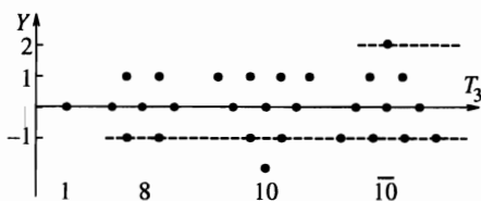
Fig. 2. T_3 - Y -diagrams for the lowest SU(3) multiplets allowed for the case of [SU(2)]^3 configurations, ansatz (11): singlet (p, q) = (0, 0) , octet (1, 1) , decuplet (3, 0) and antidecuplet (0, 3) . The lower dashed line indicates isomultiplets with Y = -1 \simeq Y_R^{min} , T = N ; the upper dashed line shows nonstrange isomultiplets with Y = B = 2
