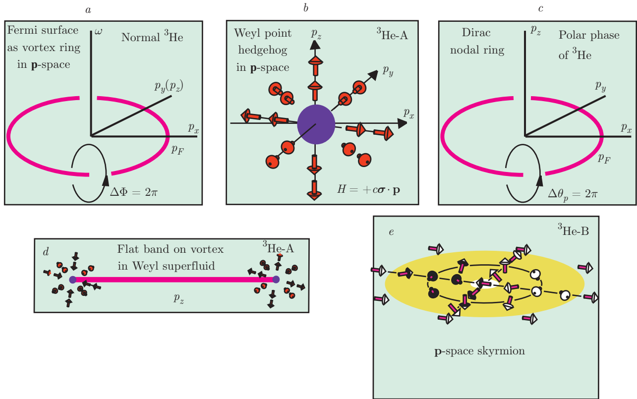
Fig. 3. Topological materials as configurations in momentum space. (a) Fermi surface in normal liquid {}^3\text{He} is topologically protected, since the Green's function has singularity in the form of the vortex ring in the (\mathbf{p}, \omega) -space. (b) Weyl point in {}^3\text{He-A} as the hedgehog in \mathbf{p} -space. It can be also represented as the \mathbf{p} -space Dirac monopole with the Berry magnetic flux. (c) The polar phase has the Dirac nodal line in \mathbf{p} -space—the counterpart of the spin vortex in real space. (d) The \mathcal{N} = \infty singular vortex in chiral superfluid {}^3\text{He-A} has the 1D flat band terminated by the projections of the Weyl points to the vortex line. In real space it has analogy with the Dirac monopole terminating the Dirac string. (e) Skyrmion configurations in \mathbf{p} -space describe the fully gapped topological superfluids. The 2D skyrmion describes the topology of the {}^3\text{He-A} state in a thin film and the topology of 2D planar phase of {}^3\text{He} . The 3D \mathbf{p} -space skyrmion describes the superfluid {}^3\text{He-B}
