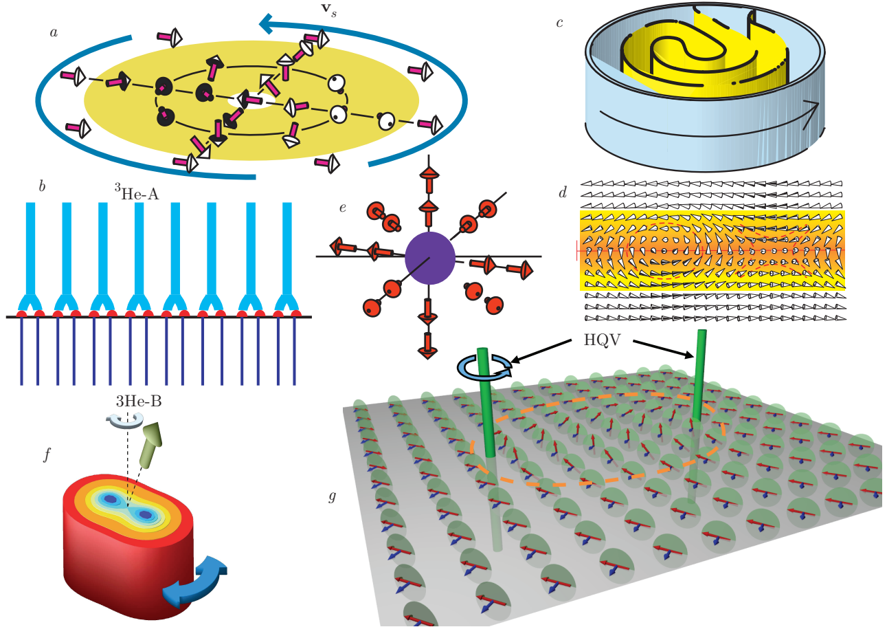
Fig. 1. (Color online) Some topological objects in topological superfluids. (a) Vortex-skyrmions with two quanta of circulation ( \mathcal{N} = 2 ) in the chiral superfluid {}^3\text{He-A} . (b) Interface between {}^3\text{He-A} and {}^3\text{He-B} in rotation: lattice of skyrmions with \mathcal{N} = 2 in {}^3\text{He-A} transforms to the lattice of singly quantized vortices ( \mathcal{N} = 1 ) in {}^3\text{He-B} . Each skyrmion with \mathcal{N} = 2 splits into two merons with \mathcal{N} = 1 (Mermin–Ho vortices). The Mermin–Ho vortex terminates on the boojum — the surface singularity which is the analog of the Dirac monopole terminating the {}^3\text{He-B} string (the \mathcal{N} = 1 vortex). (c) Vortex sheet in {}^3\text{He-A} . (d) Elements of the vortex sheet: merons with \mathcal{N} = 1 within topological soliton in {}^3\text{He-A} . (e) Hedgehog-monopole in the \hat{\mathbf{d}} -vector field in {}^3\text{He-A} . (f) Singly quantized vortex ( \mathcal{N} = 1 ) with spontaneously broken axial symmetry in {}^3\text{He-B} as a pair of half-quantum vortices ( \mathcal{N} = 1/2 ) connected by non-topological (dark) soliton. Such vortex has been identified due to Goldstone mode associated with the spontaneously broken axial symmetry of the vortex core — the twist oscillations of the vortex core propagating along the vortex line. This Figure is also applicable to the \mathcal{N} = 2 vortex in {}^3\text{He-B} , which consists of two composite objects — spin-mass vortices connected by the topological soliton. (g) Half-quantum vortices (HQP) in the polar phase of {}^3\text{He} , which in a tilted magnetic field are connected by the topological spin soliton. Red arrows show direction of magnetic field, and blue arrows show direction of spin-nematic vector \hat{\mathbf{d}} , which rotates by \pi around each half-quantum vortex
